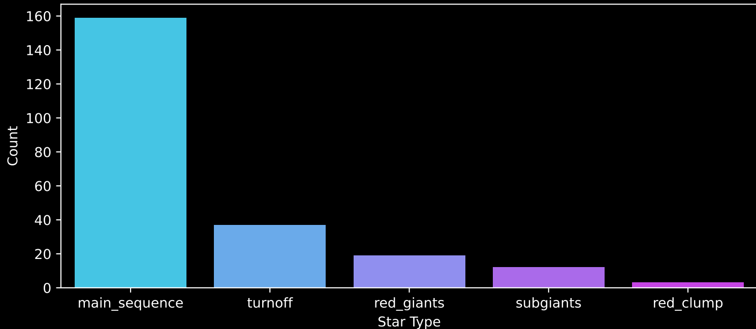
APOGEE DR17 Field: [Sgr_tidal3] Count plot of Star Type
