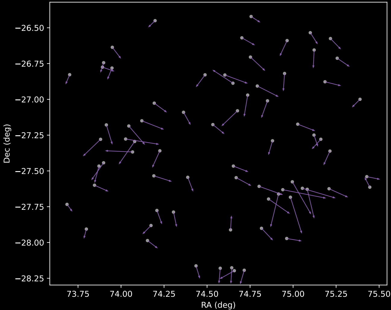
APOGEE DR17 Cluster 8 Proper Motion Vectors (n=72)
