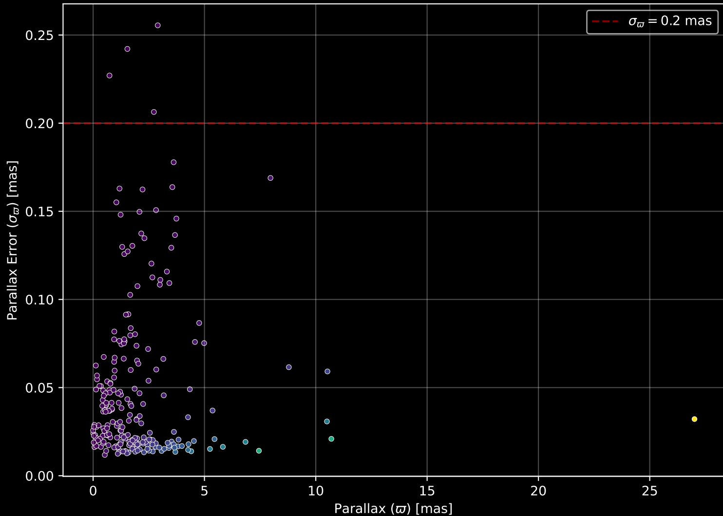
APOGEE DR17 Field: [Sgr_tidal3] Parallax Quality (n= 230)
