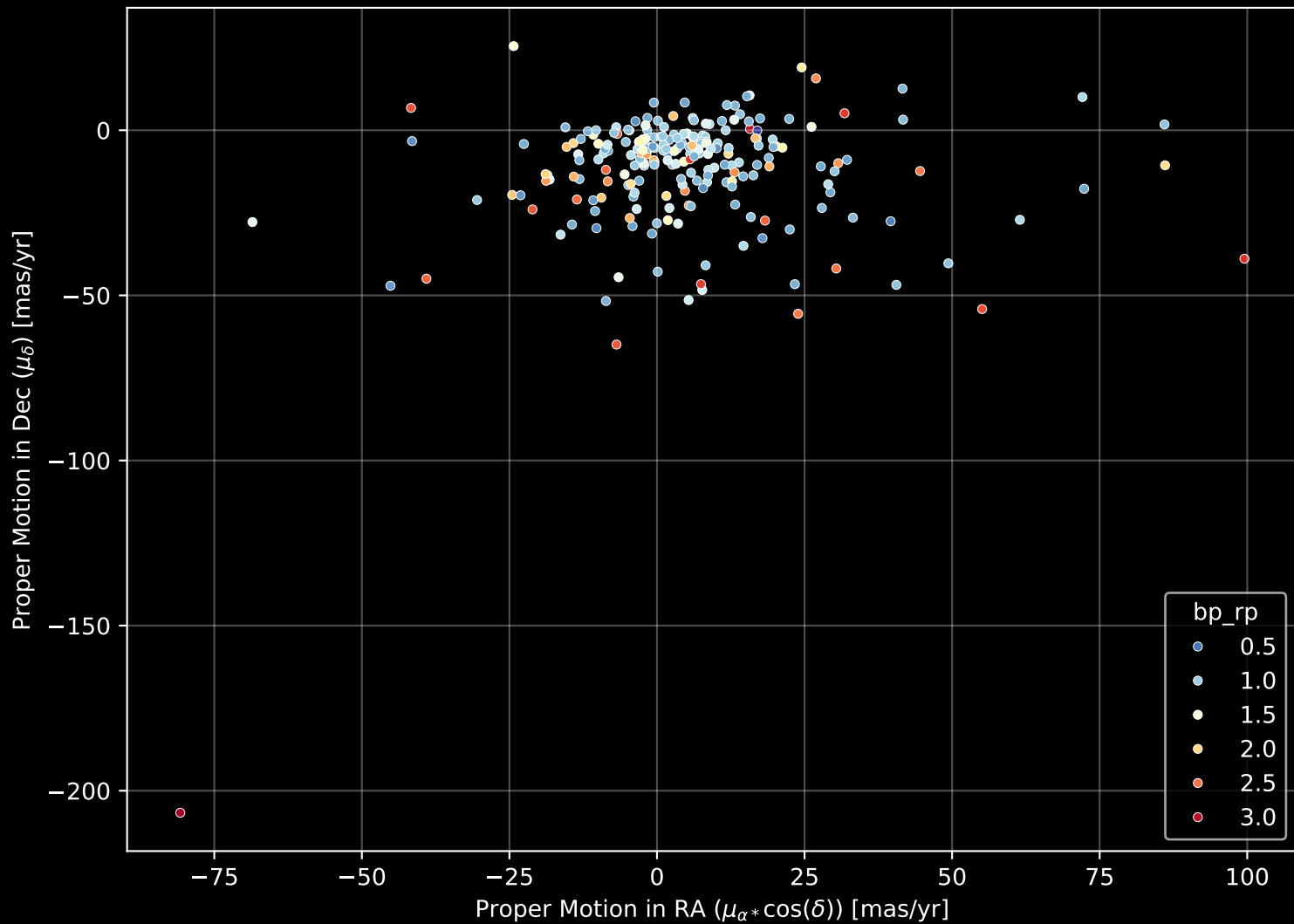
APOGEE DR17 Field: [Sgr_tidal3] Proper Motion Diagram (n= 230)
