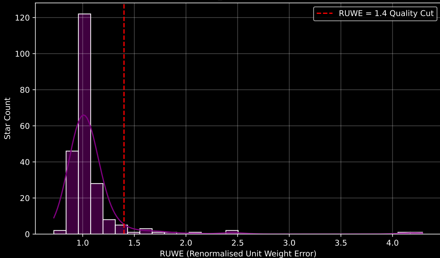
GAPOGEE DR17 Field [Sgr_tidal3] RUWE Distribution (n= 222)
