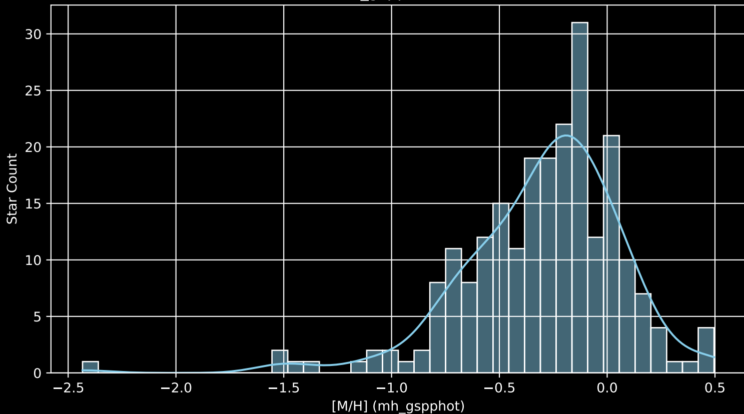
APOGEE DR17 Field: [Sgr_tidal3 [M/H] (mh_gspphot) (n= 229)
